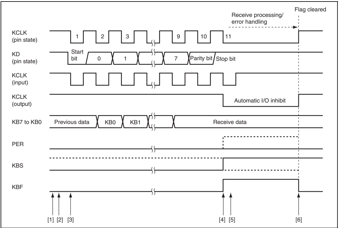
Figure 14.4 Receive Timing
